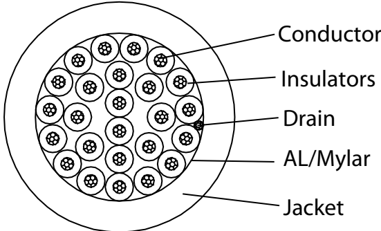
Cable Sectional
