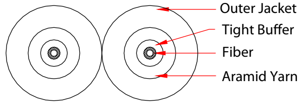
Cross Section
