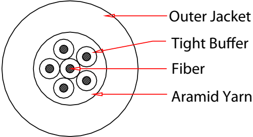
Cross Section
