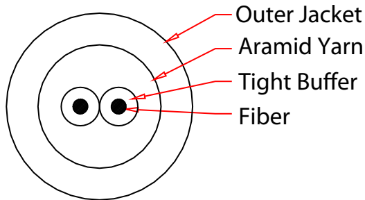
Cable Section
