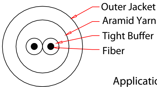
Cable Section
