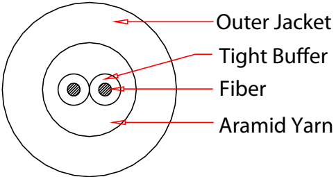
Cross Section
