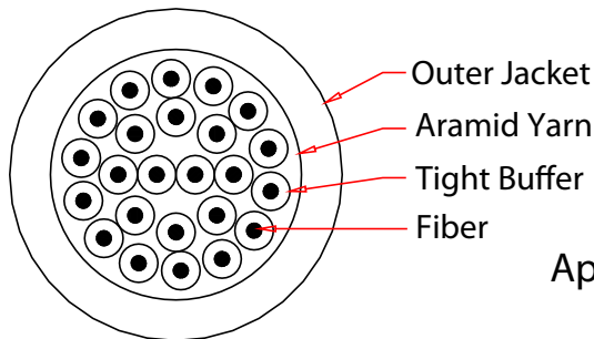
Cable Section
