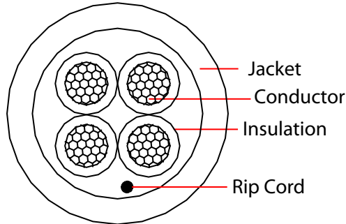
Cross Section
