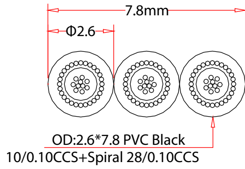
Cable Cross Section
