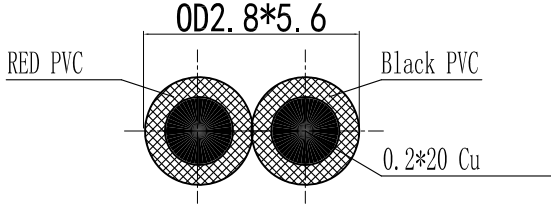
CABLE CONSTRUCTION
