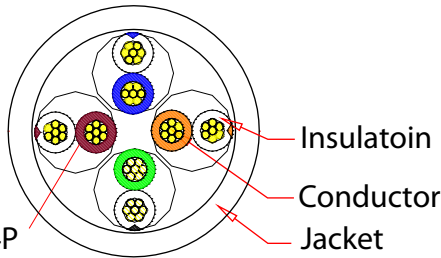
Cable Cross-Section
