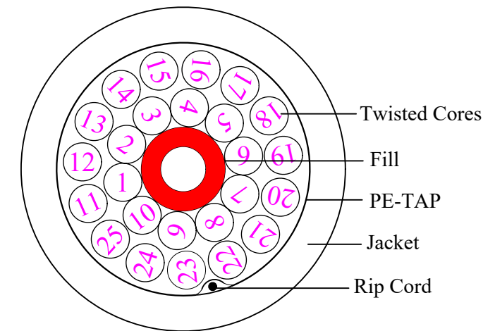
Cross Section
