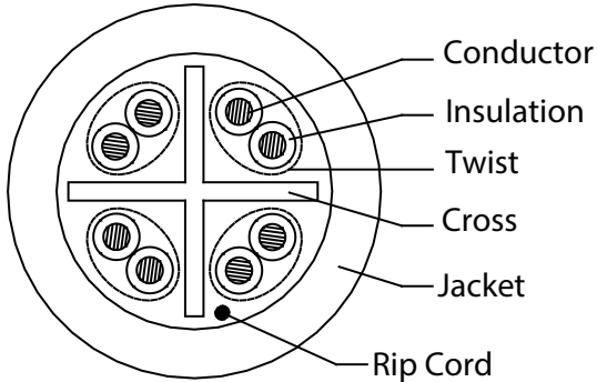
Cross Section
