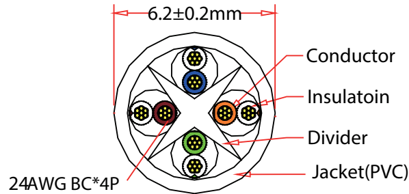
Cable Cross-Section
