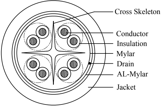
Cross Section
