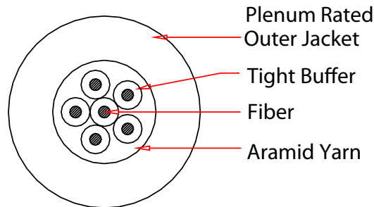
Cross Section
