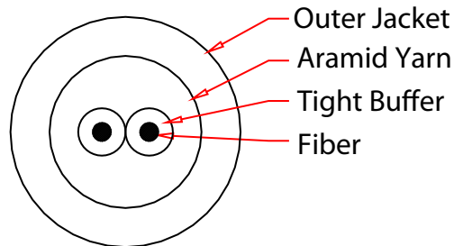
Cable Section
