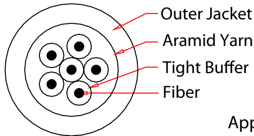
Cable Section
