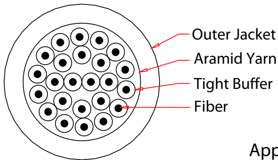
Cable Section
