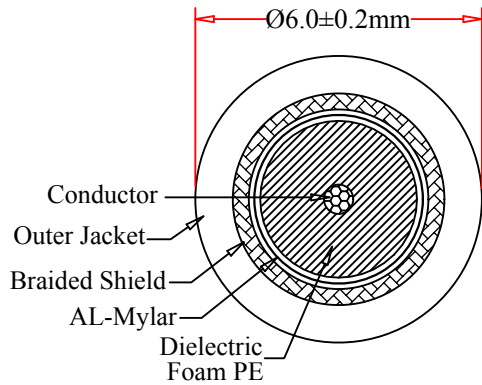
Cable Section
