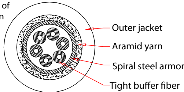
Cross Section
