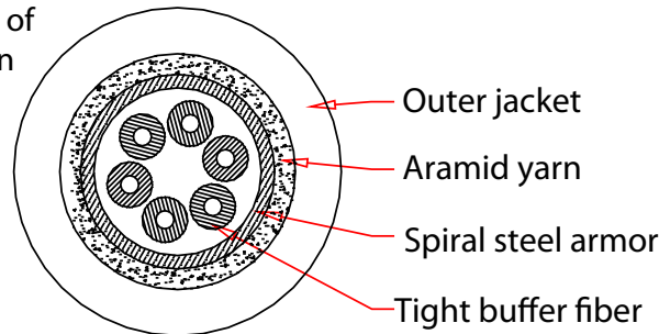
Cross Section
