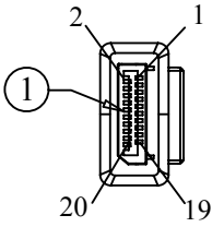
DP Male
