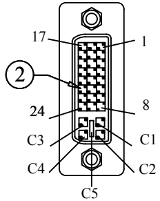
DVI (24+5) Female
