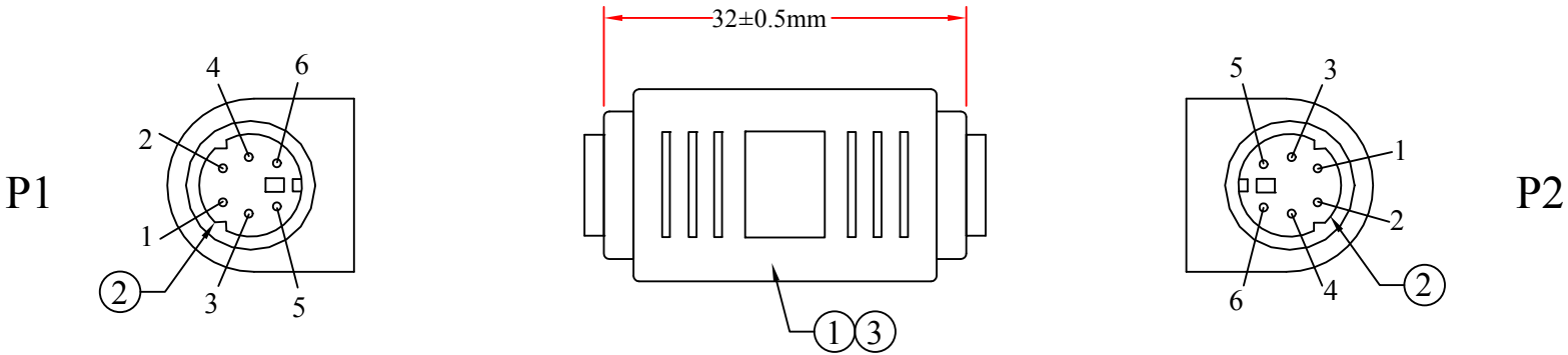
Mini Din 6P (PS/2) Female to Female
