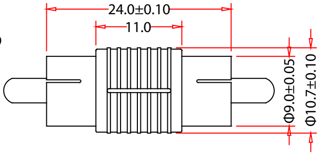
RCA Male to RCA Male, Nickel Plated
