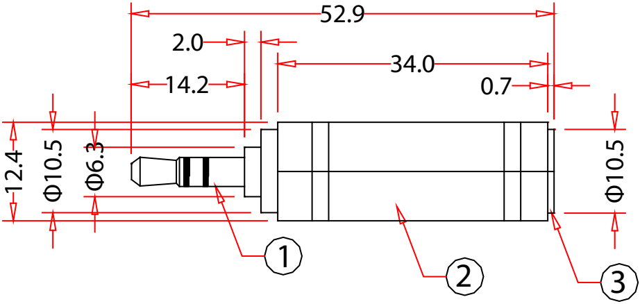
3.5mm Stereo Male to 1/4 inch(6.35mm) Stereo Female Adapter
