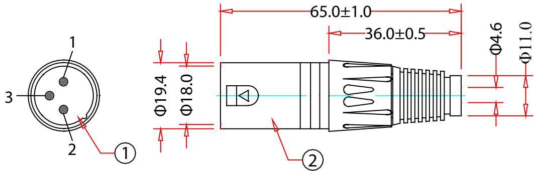
XLR 3P Microphone Connector Male
