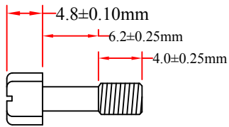
SCREW
