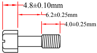
SCREW
