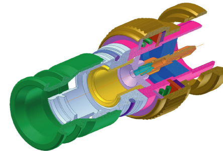
BNC Compression Connector, Nickel Plated
