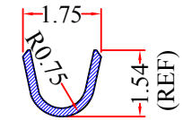
Y-Y STION
