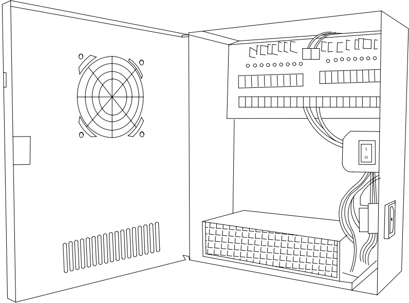
12V DC Power Distribution Box with Circulation Window, 18 Ports, 18 Amps, PTC Fuses, UL / cUL
