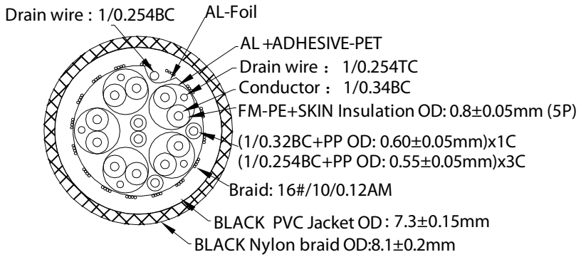
Cable Section
