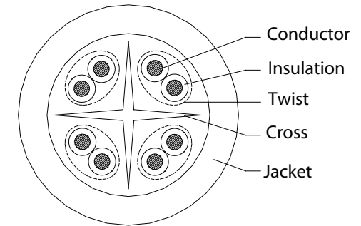
Cross Section
