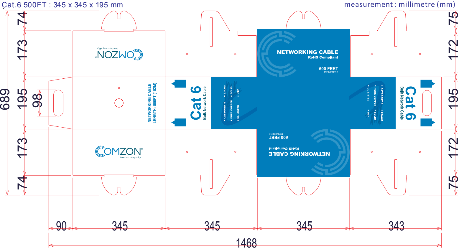
Pullbox Size
