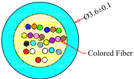
Cable Structure
