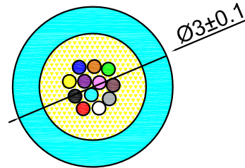
Cable Structure (Scale 10:1)
