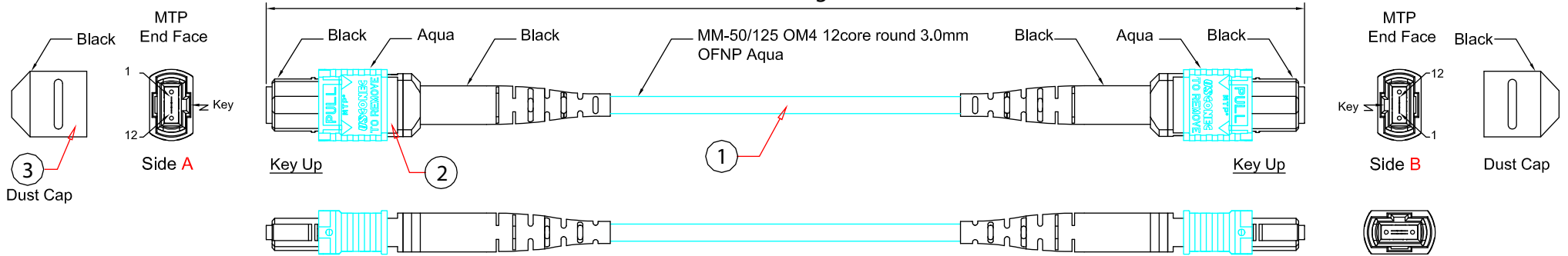
Cable Structure (Scale 10:1)
